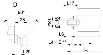
Female thread
