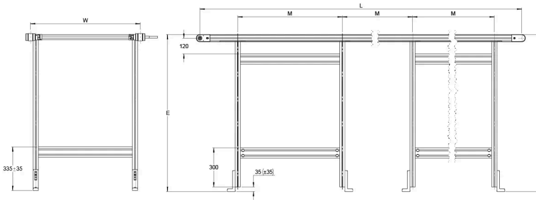
Stand TB40 Double Timing Belt Conveyor 900 < E,D ≤ 1200
