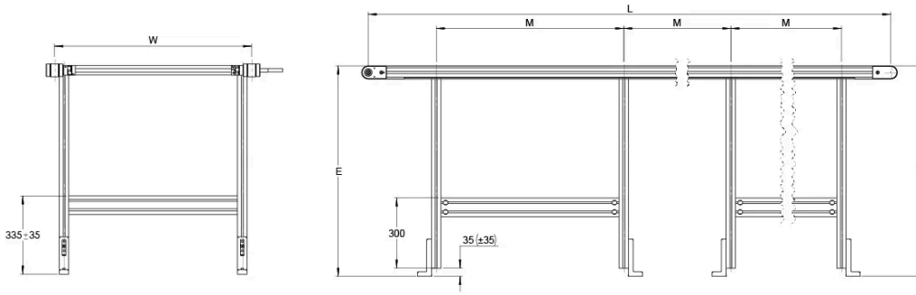
Stand TB40 Double Timing Belt Conveyor 650 < E,D ≤ 900
