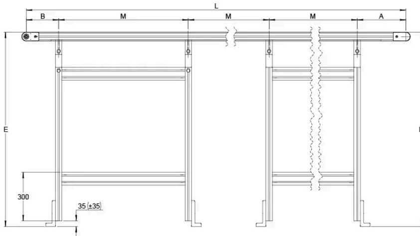
Stand TB40 Multi Timing Belt Conveyor 900 < E, D \leq 1200
